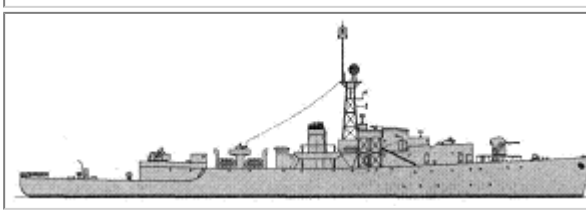
2260t, 93.6x11.8x3.8m, 2b,2vte, 5500hp, 19.5kts, 177p; 1x1-102/45, 1x4-40/39, (2x2+2x1)-20/70, 2x3-305Squid, 2DCT, 1DCR; radar: type277, 291, sonar
